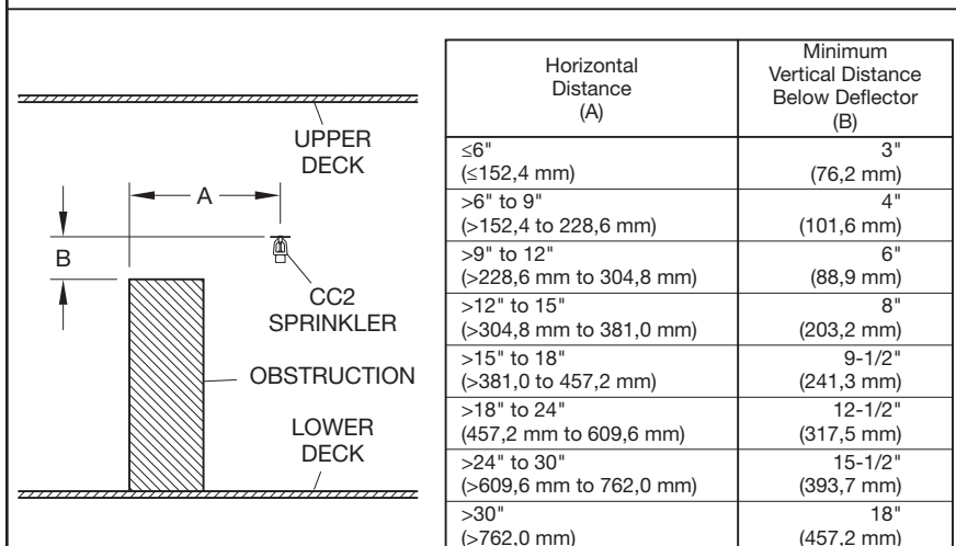
FIGURE 8 NFPA 13 OBSTRUCTION TO WATER DISTRIBUTION CRITERIA (REFERENCE)
